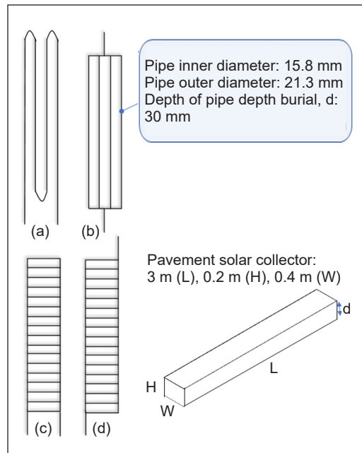
Figure 4. Pipe dimension and configuration: (a) Serpentine; (b) parallel; (c) ladder; and (d) balanced ladder
